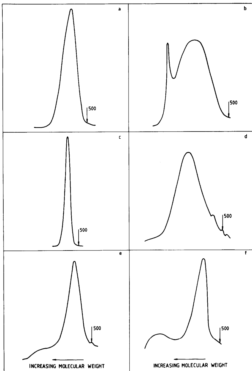
Fig. 2. Curves representing the types of MW distributions observed for tannin peracetates.
