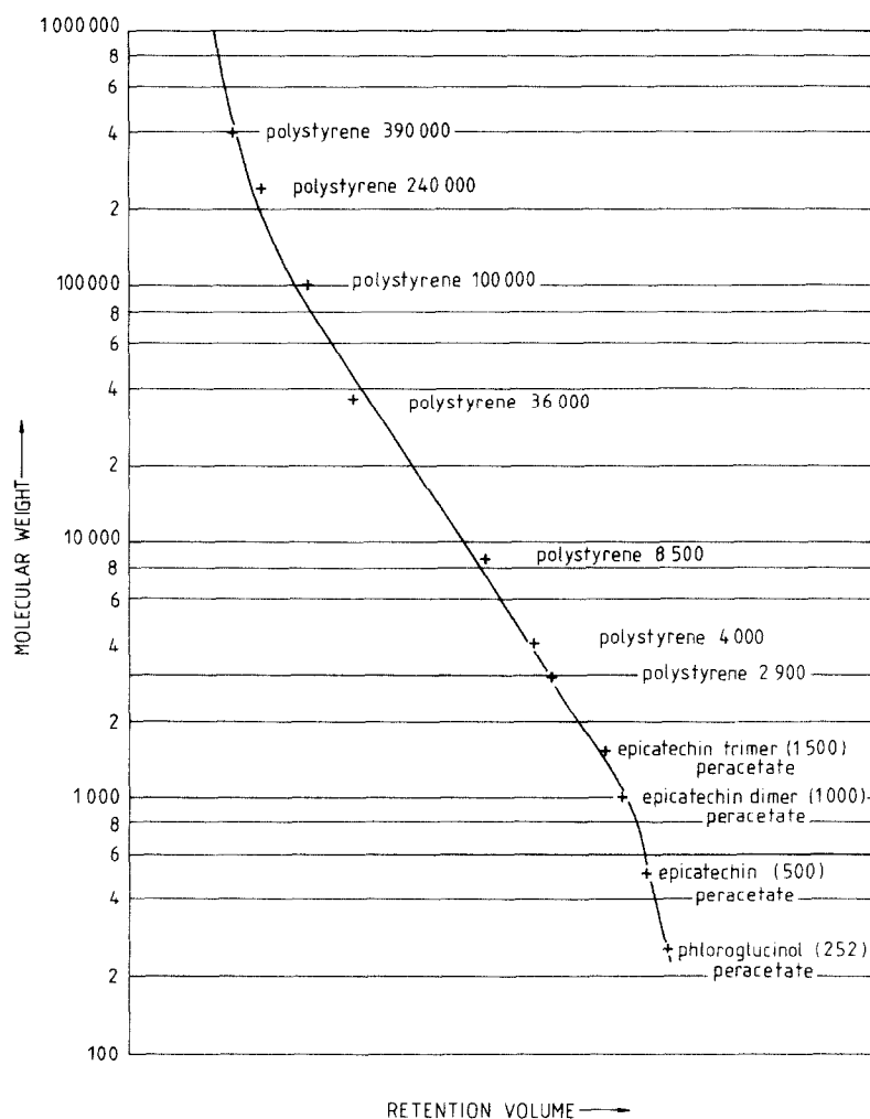
Fig. 1. Typical calibration curve for a 10^4 and 10^3 Å \mu Styragel column combination using THF as solvent.
